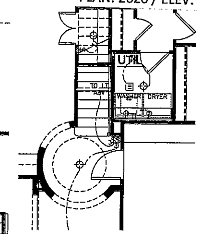
OPT 1ST FLOOR STAIRS SCALE: 11x17 1/8" = 1'-0" 34x22 1/4" = 1'-0"
