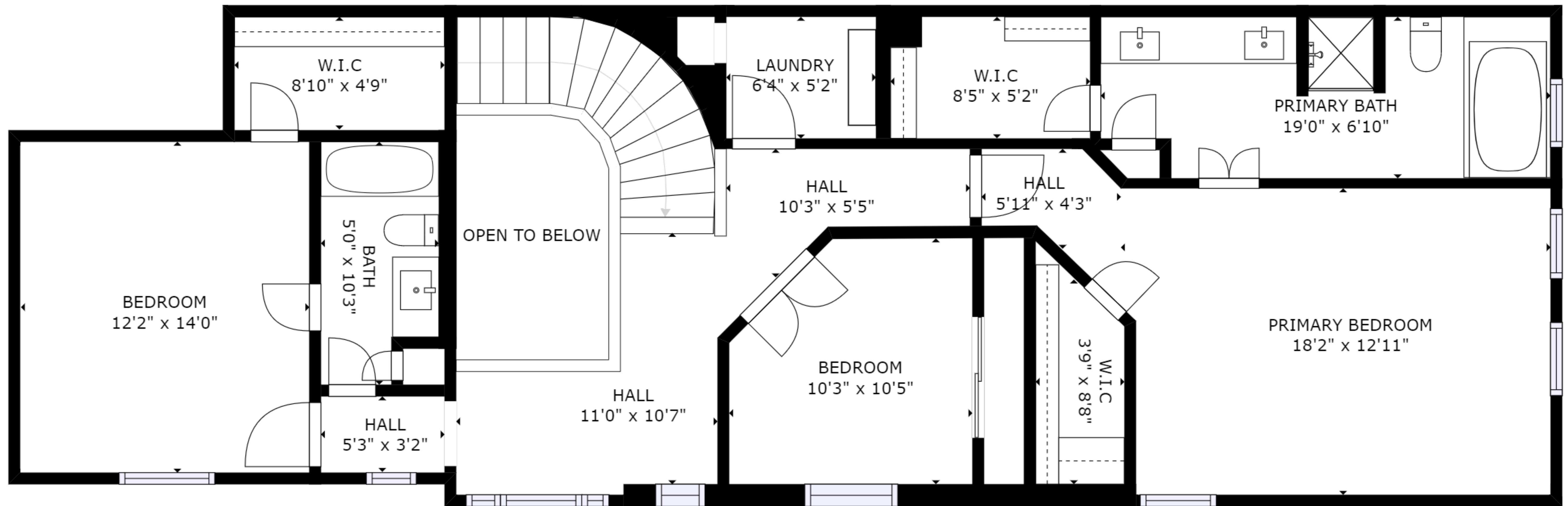
FLOOR 2
