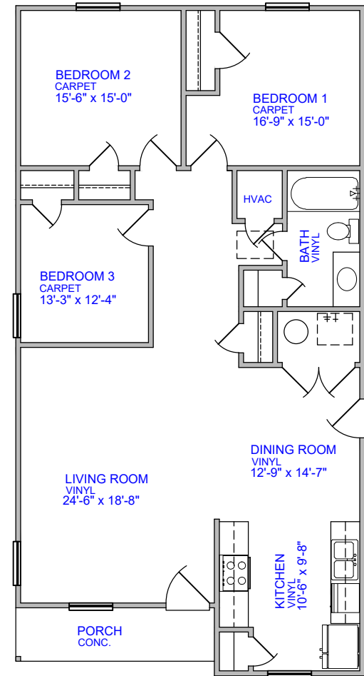
FLOOR PLAN
