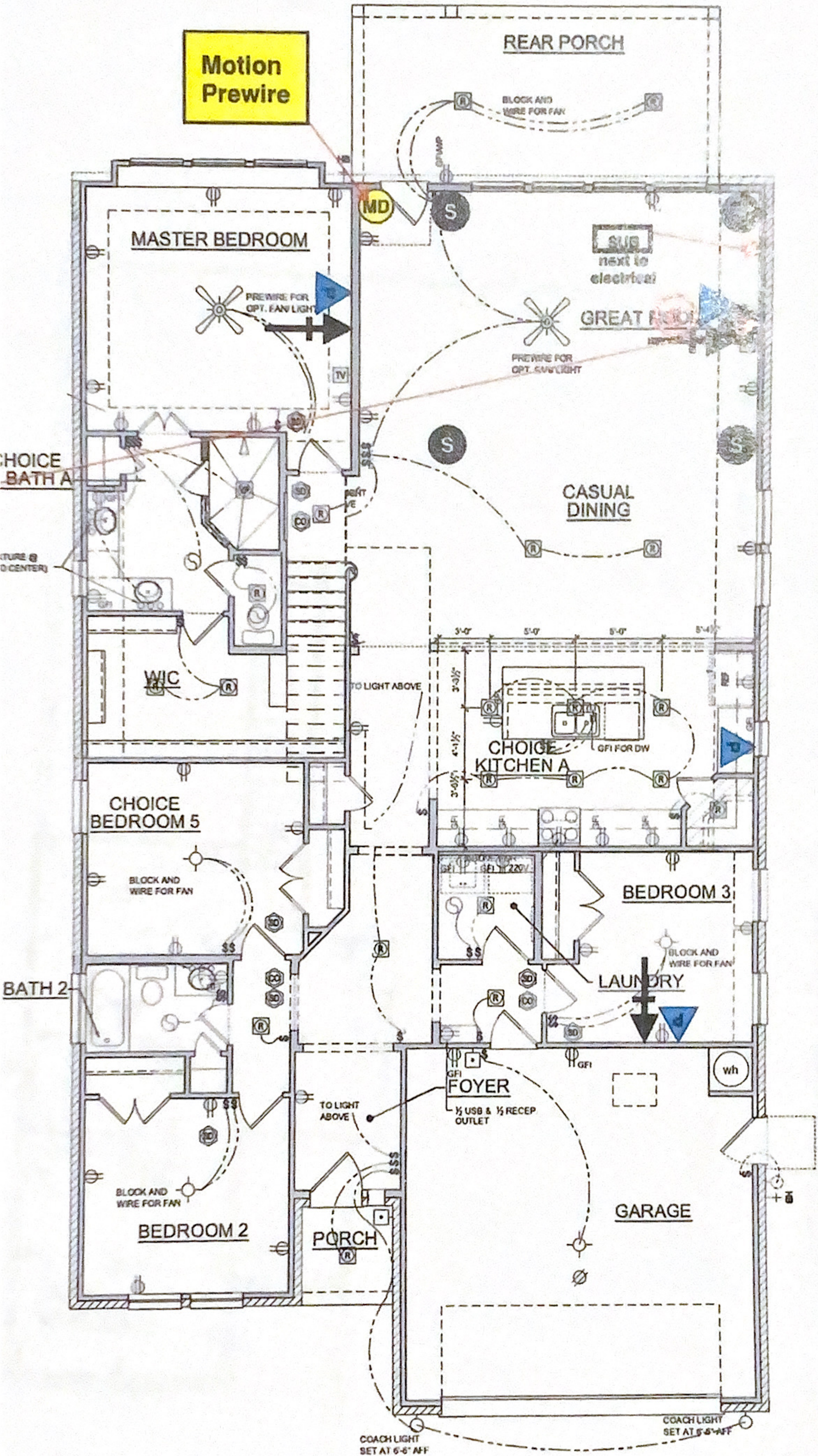
① FIRST FLOOR PLAN ELEC. PLAN - TRL SCALE: 1/8"=1'-0" (11"x17" SHEET SIZE) SCALE: 1/4"=1'-0" (24"x36" SHEET SIZE)
