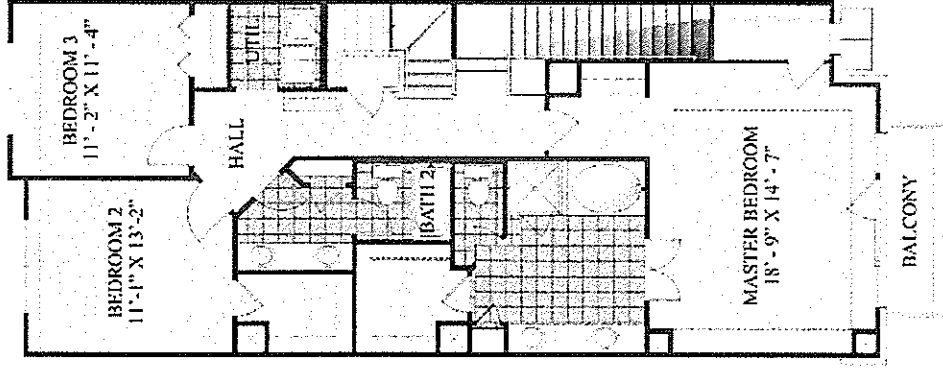
Second Floor
