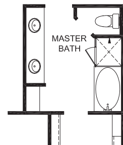
OPTIONAL 36 X 60 TUB/ 36 X 36 SHOWER AT MASTER BATH
