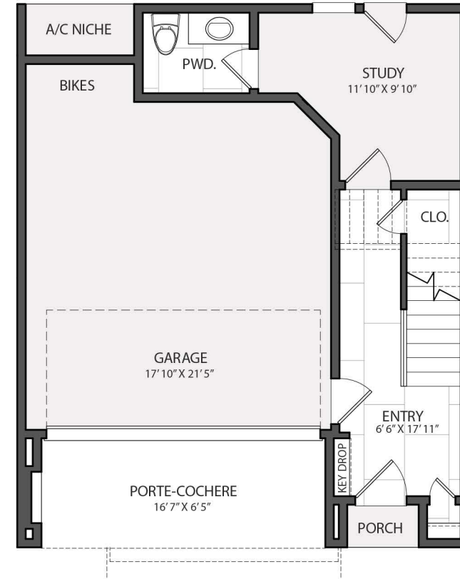
FIRST FLOOR 317 SQFT
