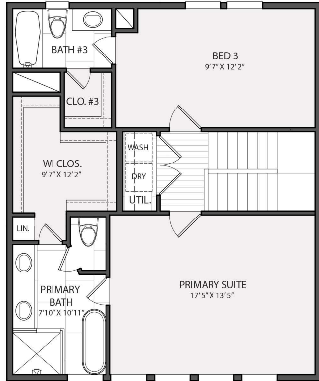
THIRD FLOOR 775 SQFT
