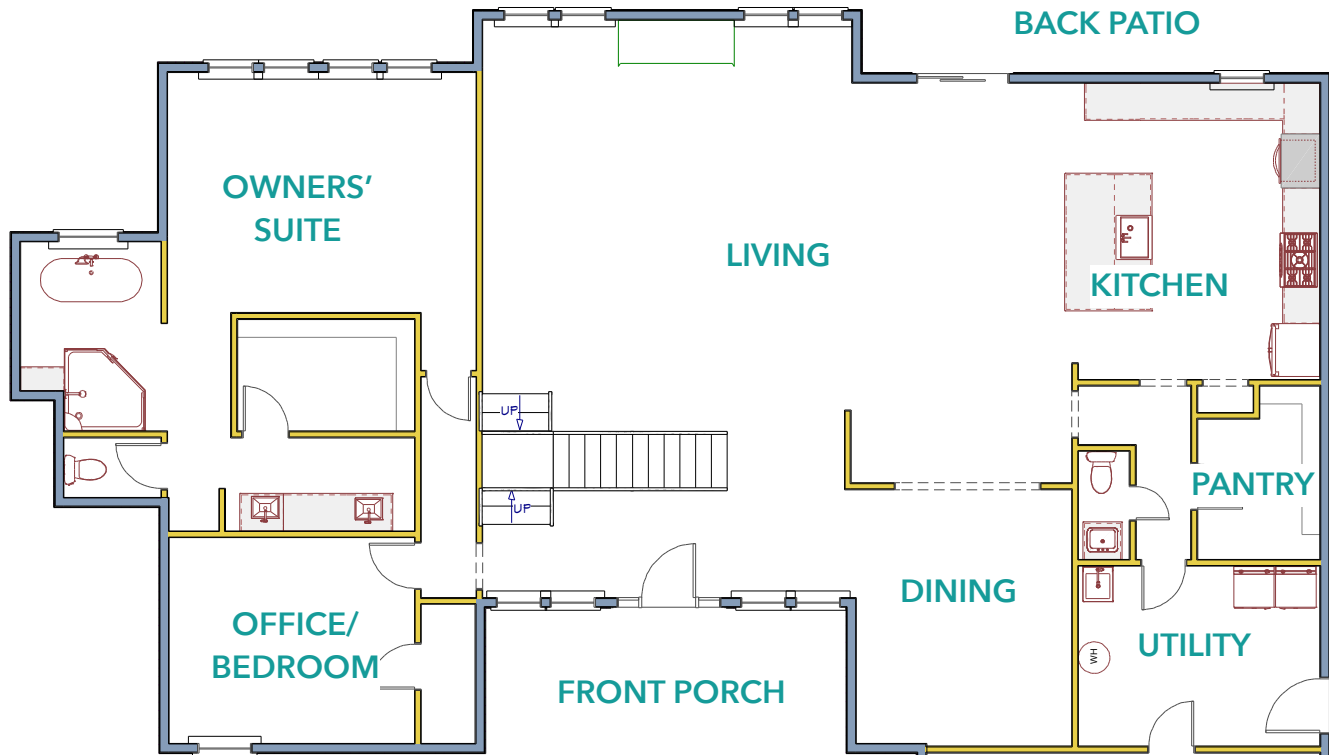
FIRST FLOOR
