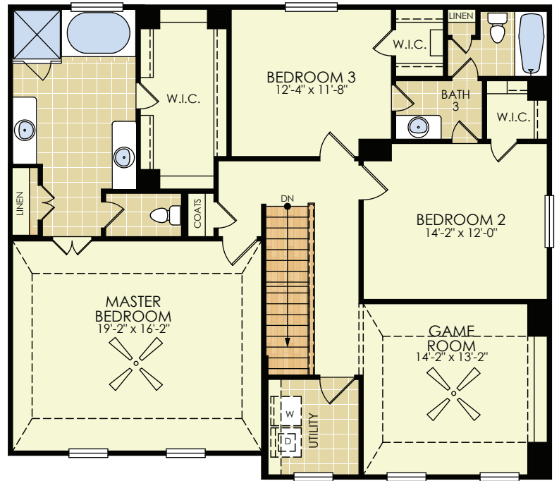
SECOND FLOOR
