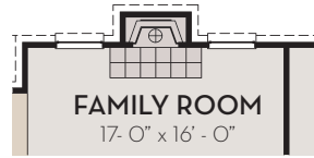
OPT. FIREPLACE
