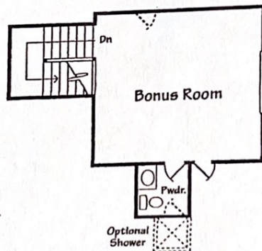
OPTIONAL THIRD FLOOR 903.3
