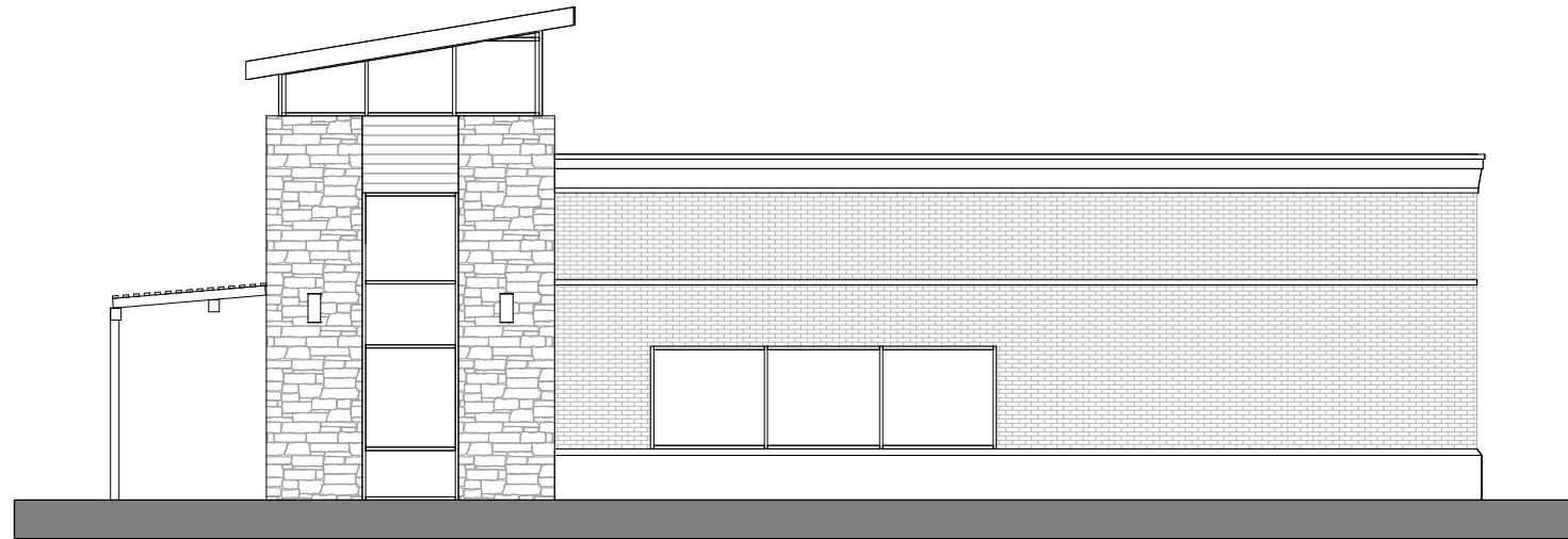
EAST ELEVATION
