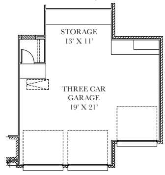
OPT. 3 CAR GARAGE W/ STORAGE
