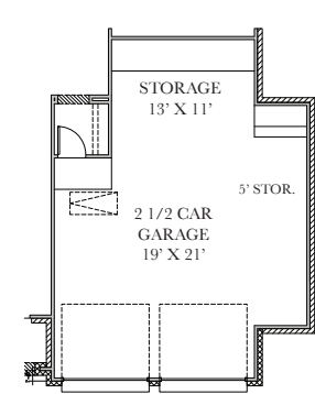
OPT. 2 1/2 CAR GARAGE W/ STORAGE
