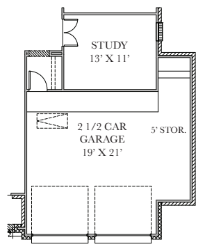
OPT. 2 1/2 CAR GARAGE W/ STUDY
