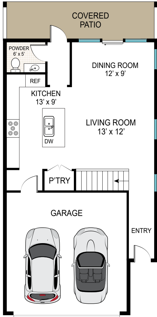
1ST FLOOR
