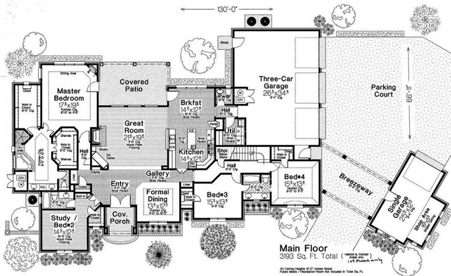
Plan Number 66248 | Order Code: 00WEB | First Floor Plan
