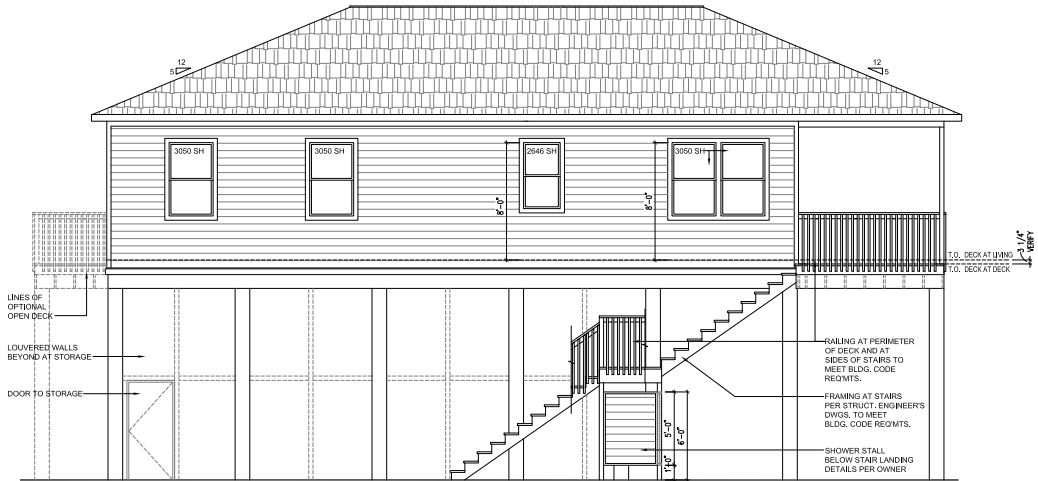
LEFT ELEVATION
