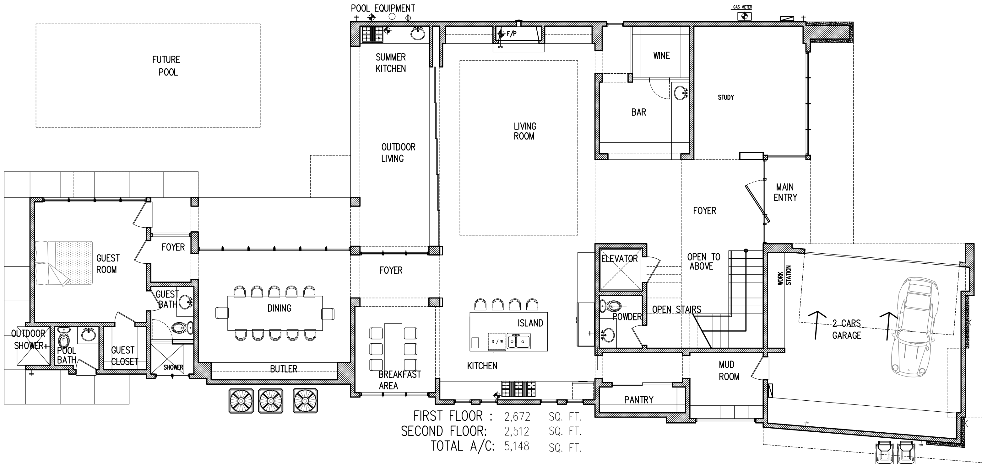
3766 PURDUE ST - FIRST FLOOR PLAN
