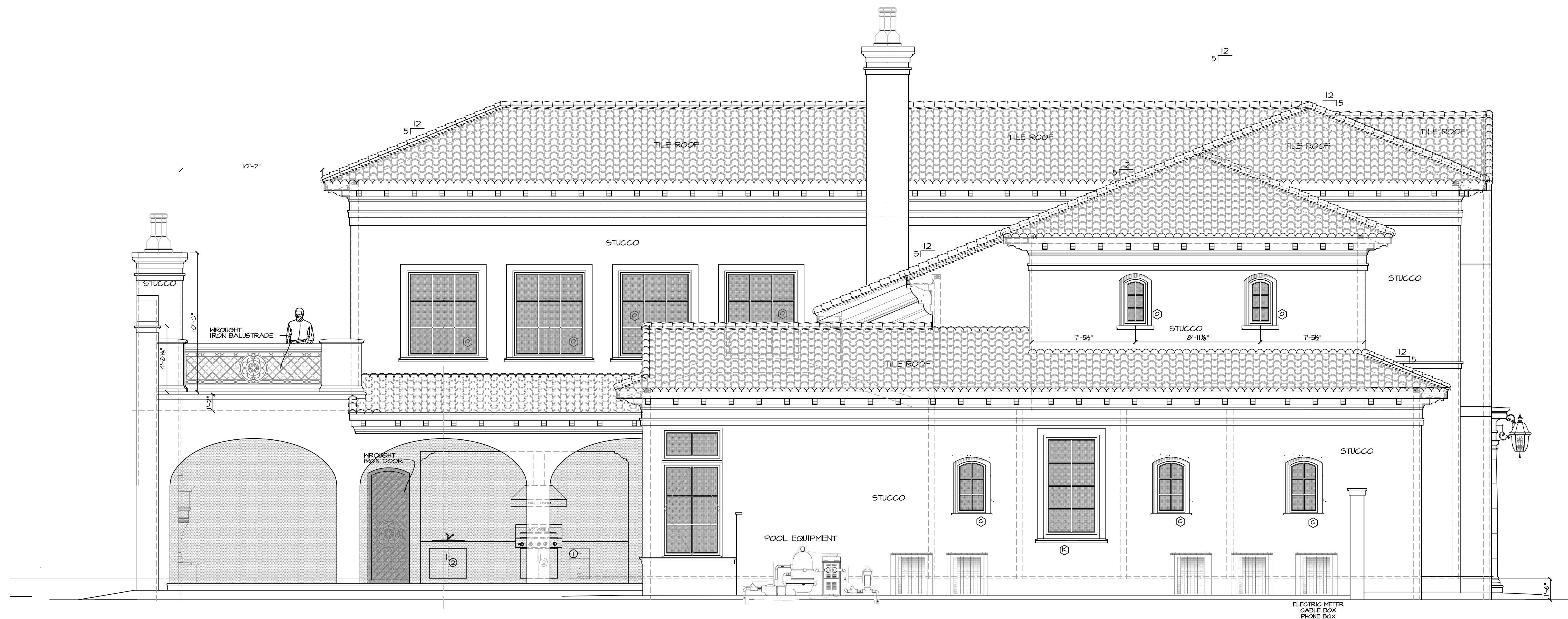
LEFT ELEVATION
