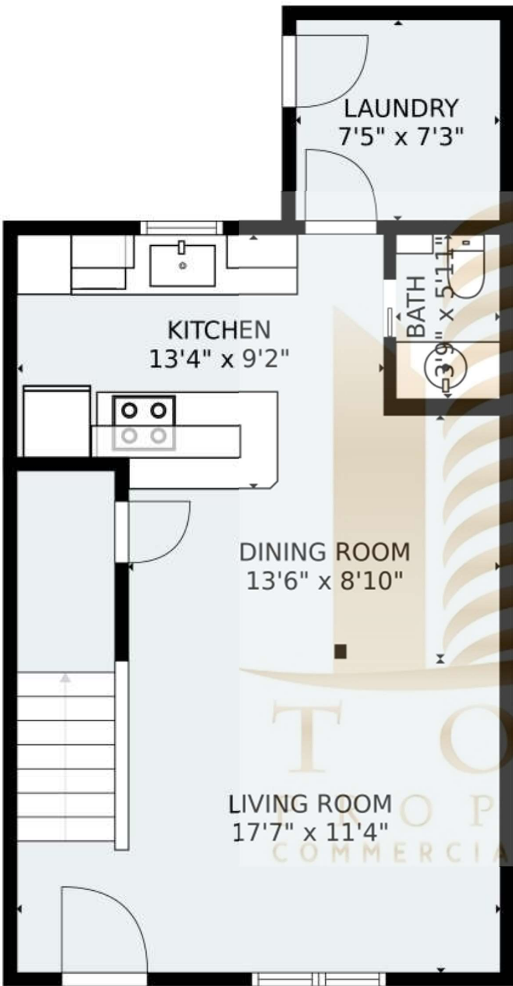
FLOOR 1
