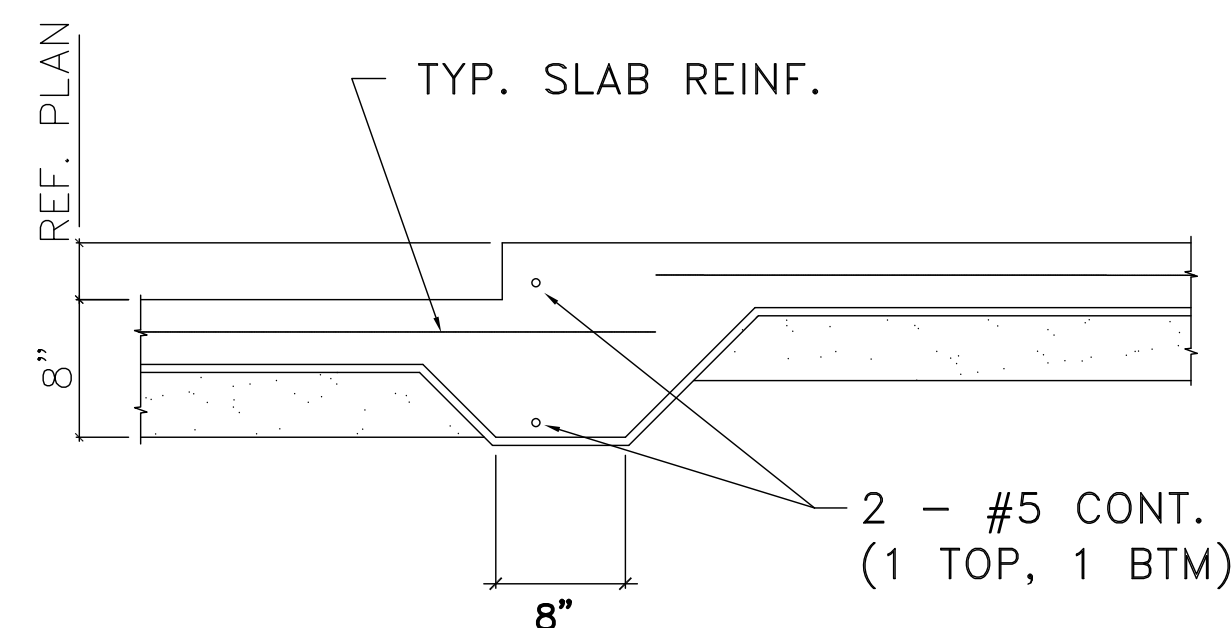
N - N Wheelstop
