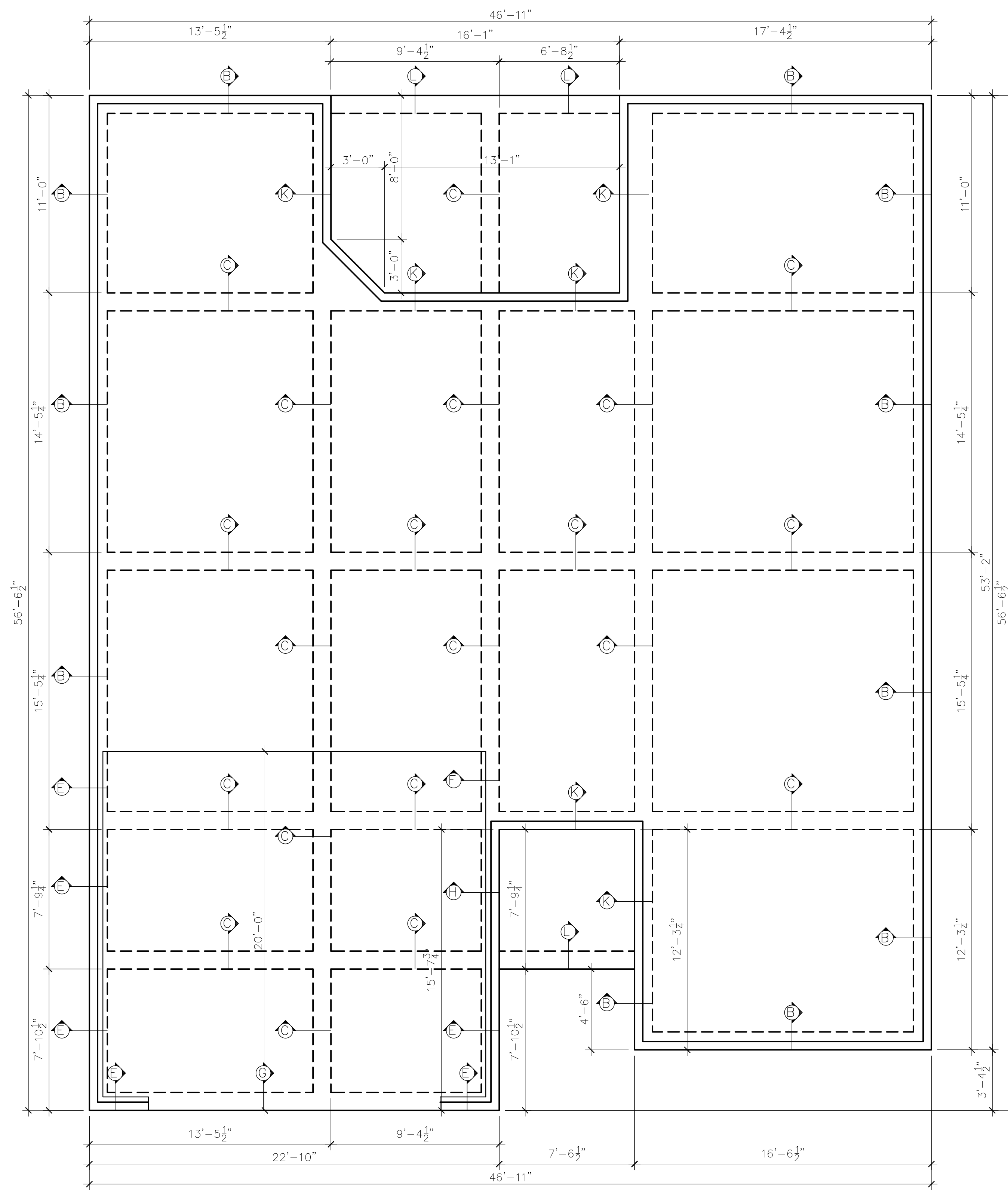
1 FOUNDATION S1 SCALE: 1/4" = 1'
