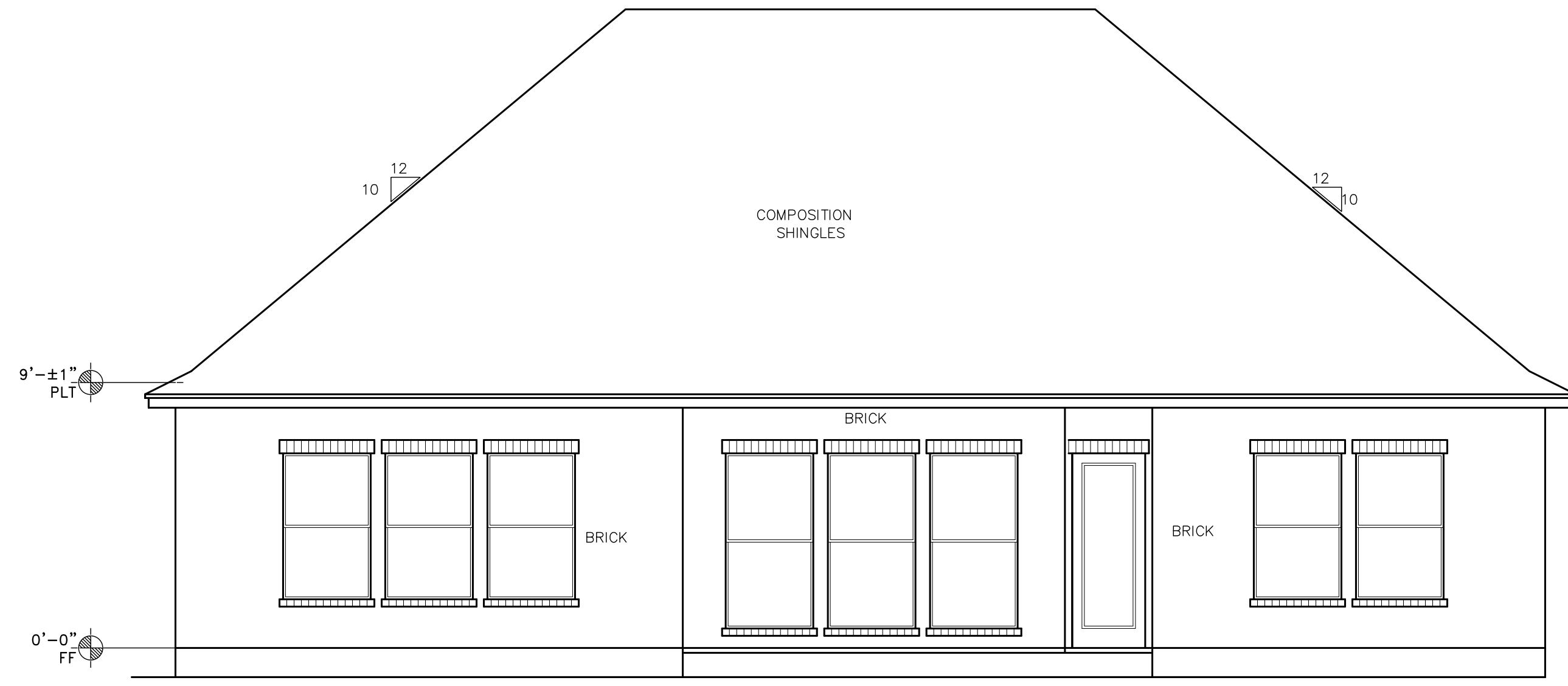
1 REAR VIEW A2 SCALE: 1/4" = 1'
