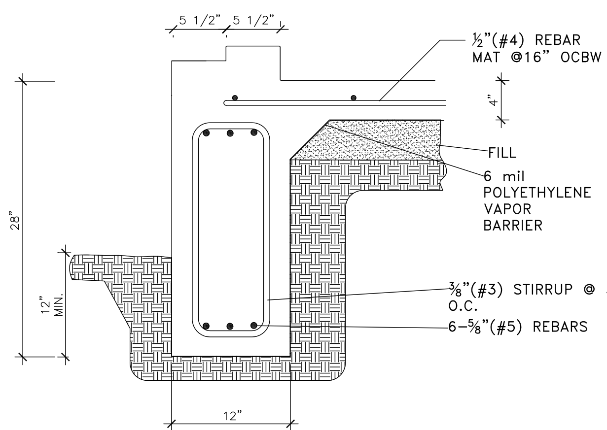
E - E PERIMETER BEAM with BRICK LEDGE
