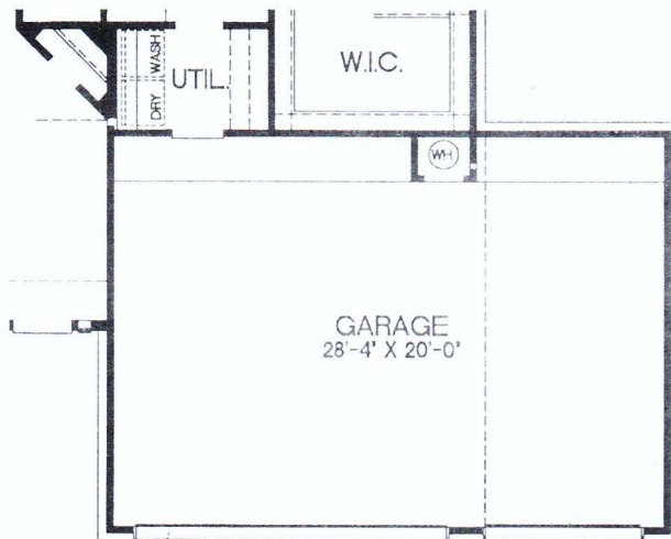
OPTIONAL 3RD CAR GARAGE
