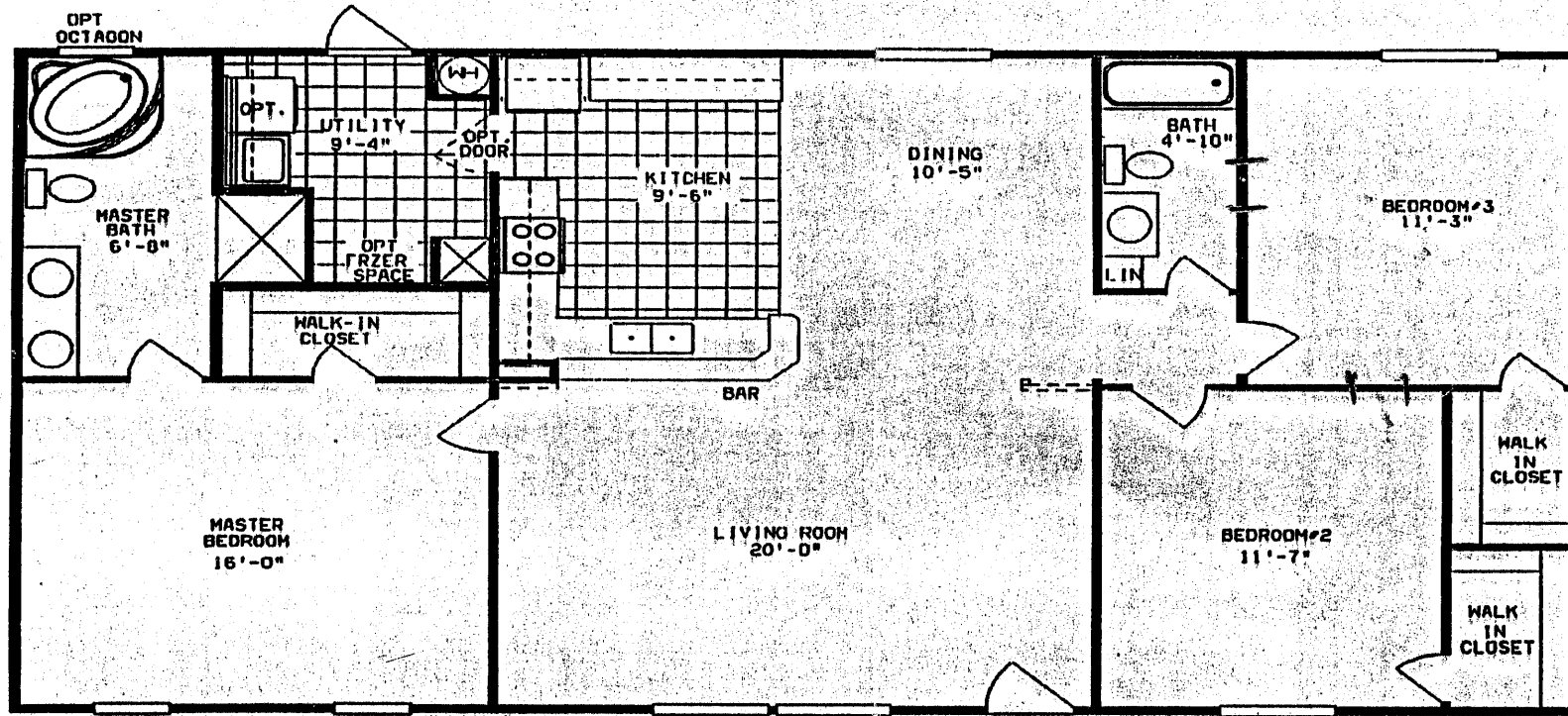
MODEL 7298 32 X 56 3 Bedroom
