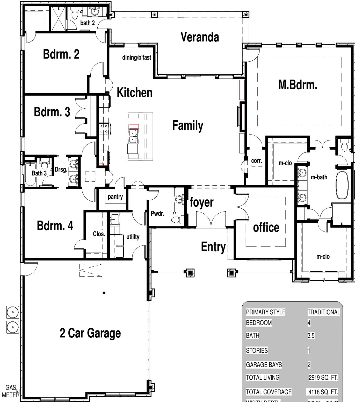
1 FLOOR PLAN - brochure
