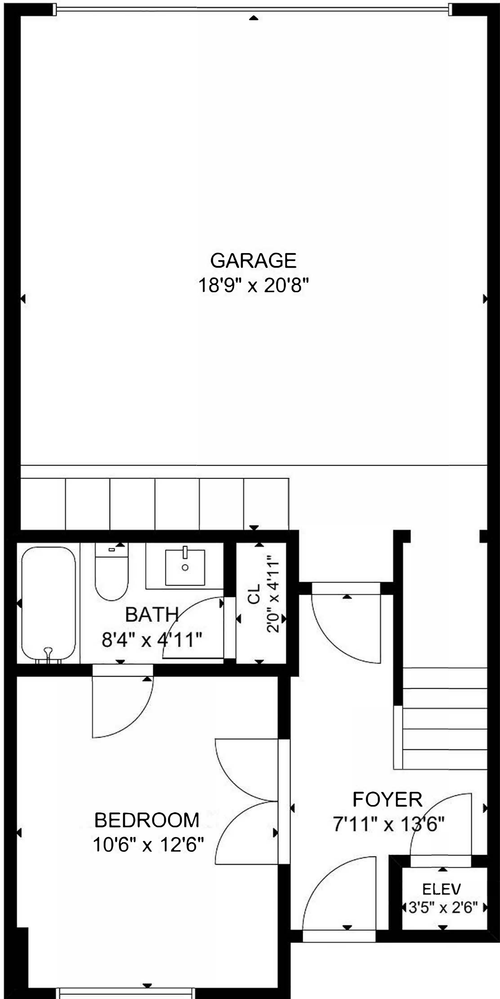
FLOOR 1
