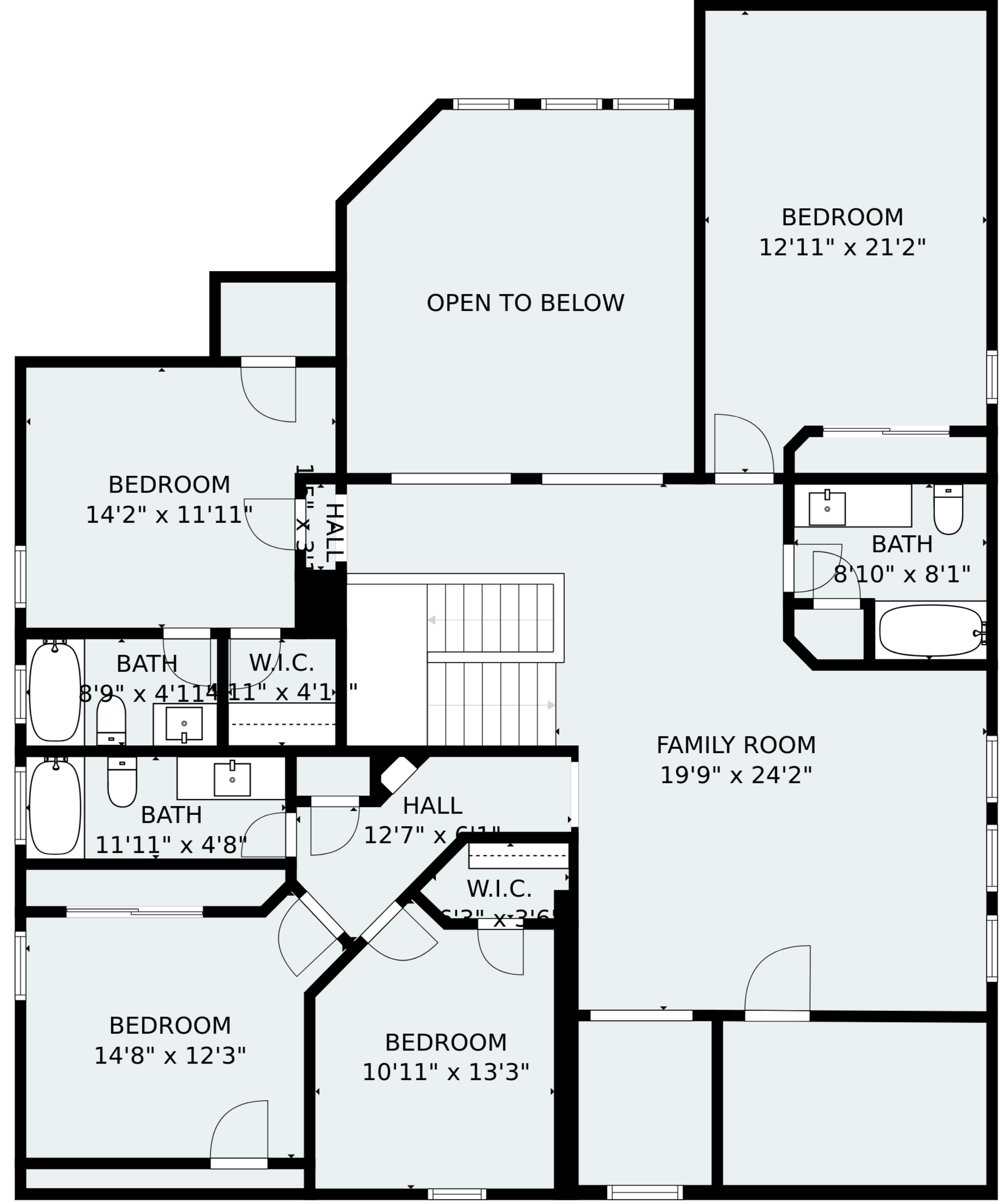
FLOOR 2
