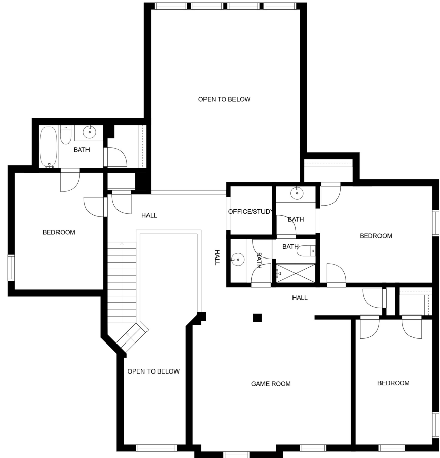
FLOOR 2
