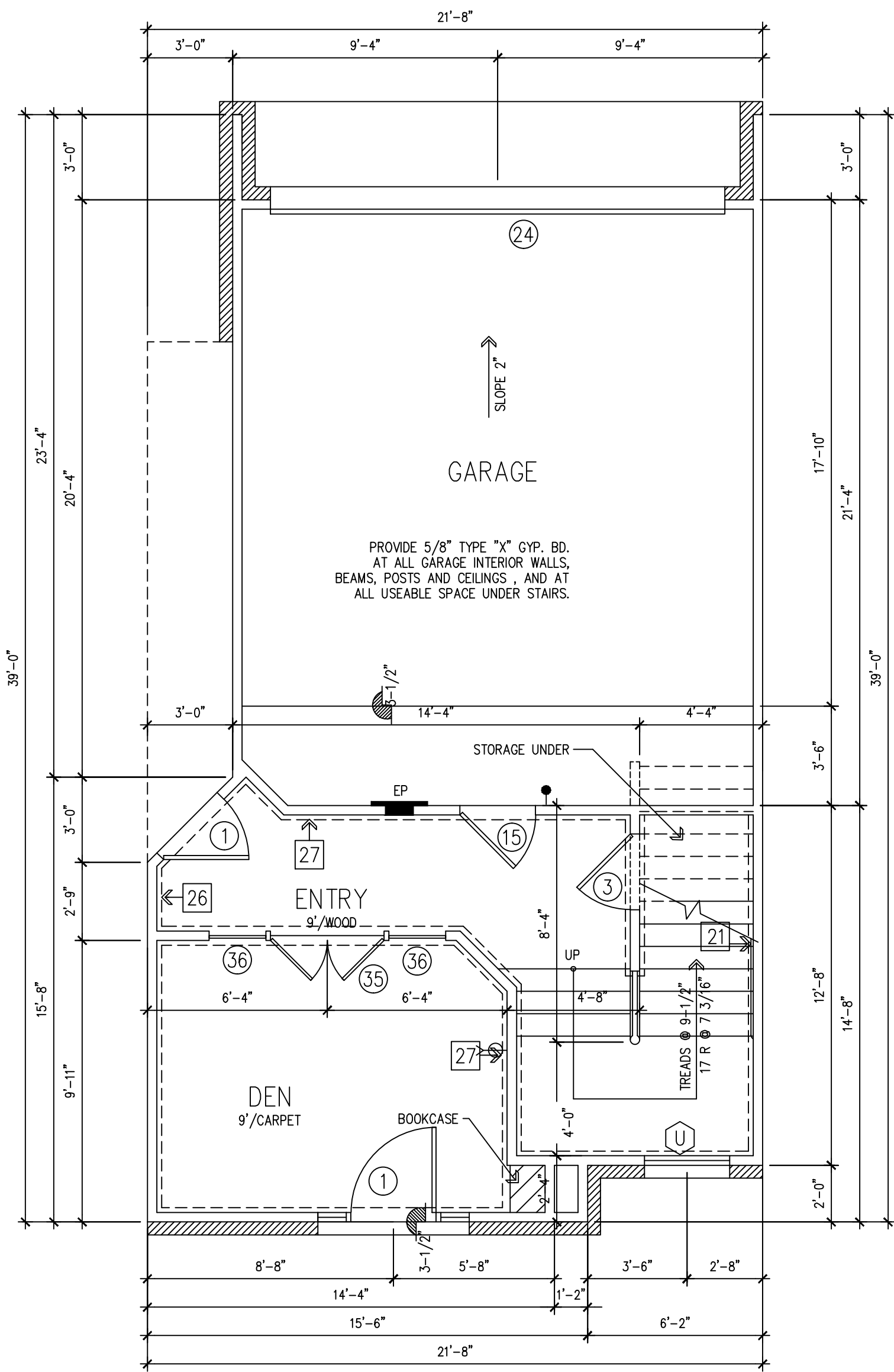
FIRST FLOOR PLAN ELEV. 1 Scale: 1/4" Date: 6-30-11
