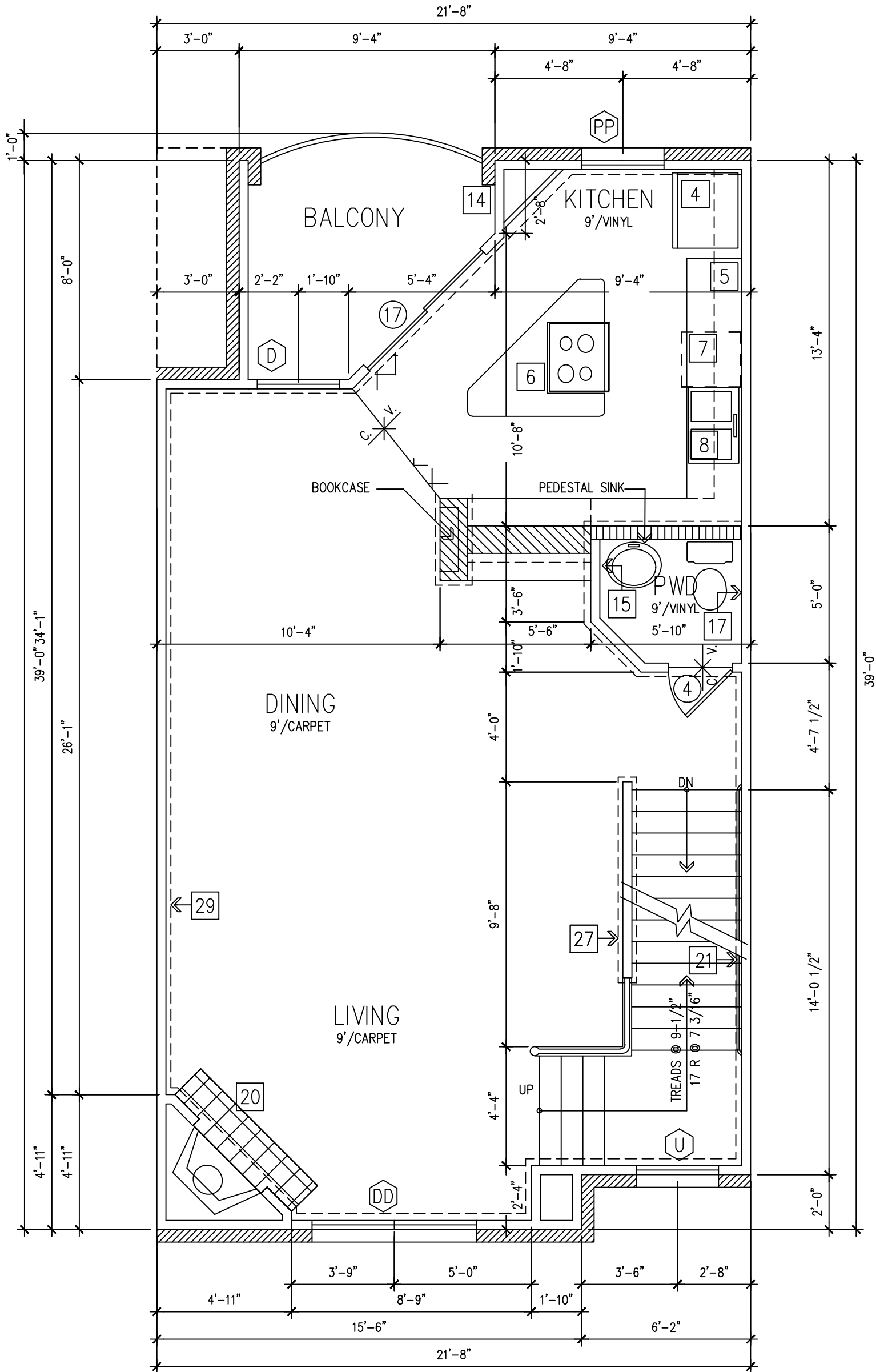
SECOND FLOOR PLAN ELEV. 1 Scale: 1/4" Date: 6-30-11
