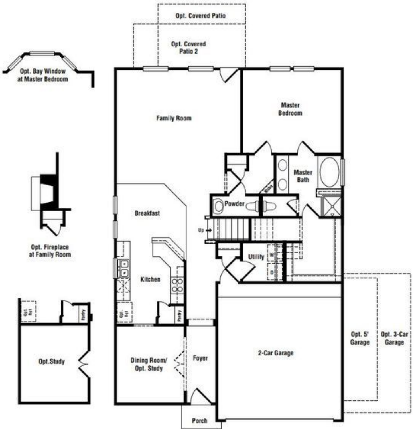
FIRST FLOOR
