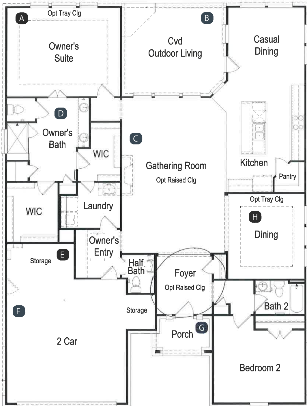
FIRST FLOOR
