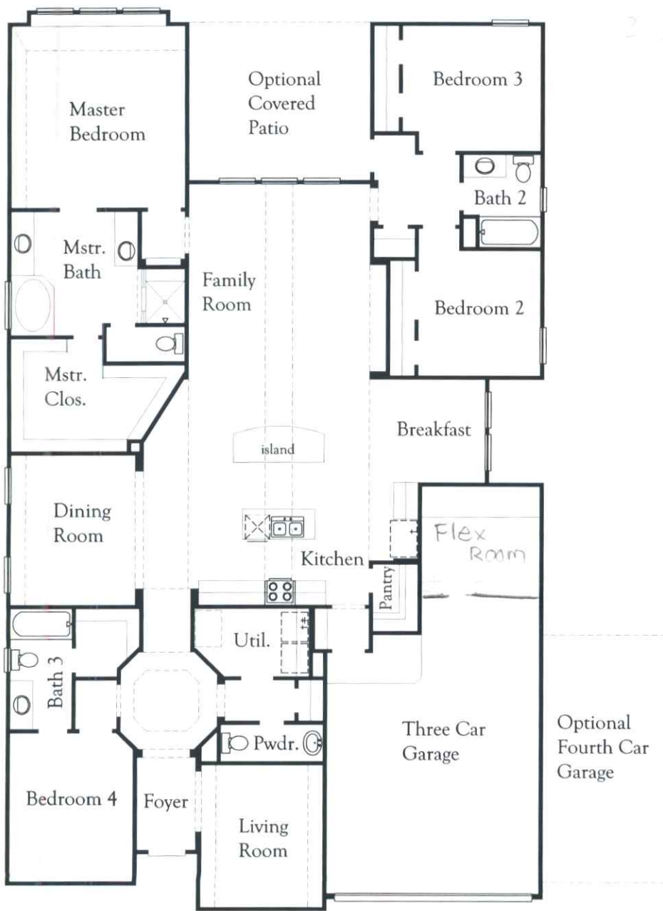
Floor Plan
