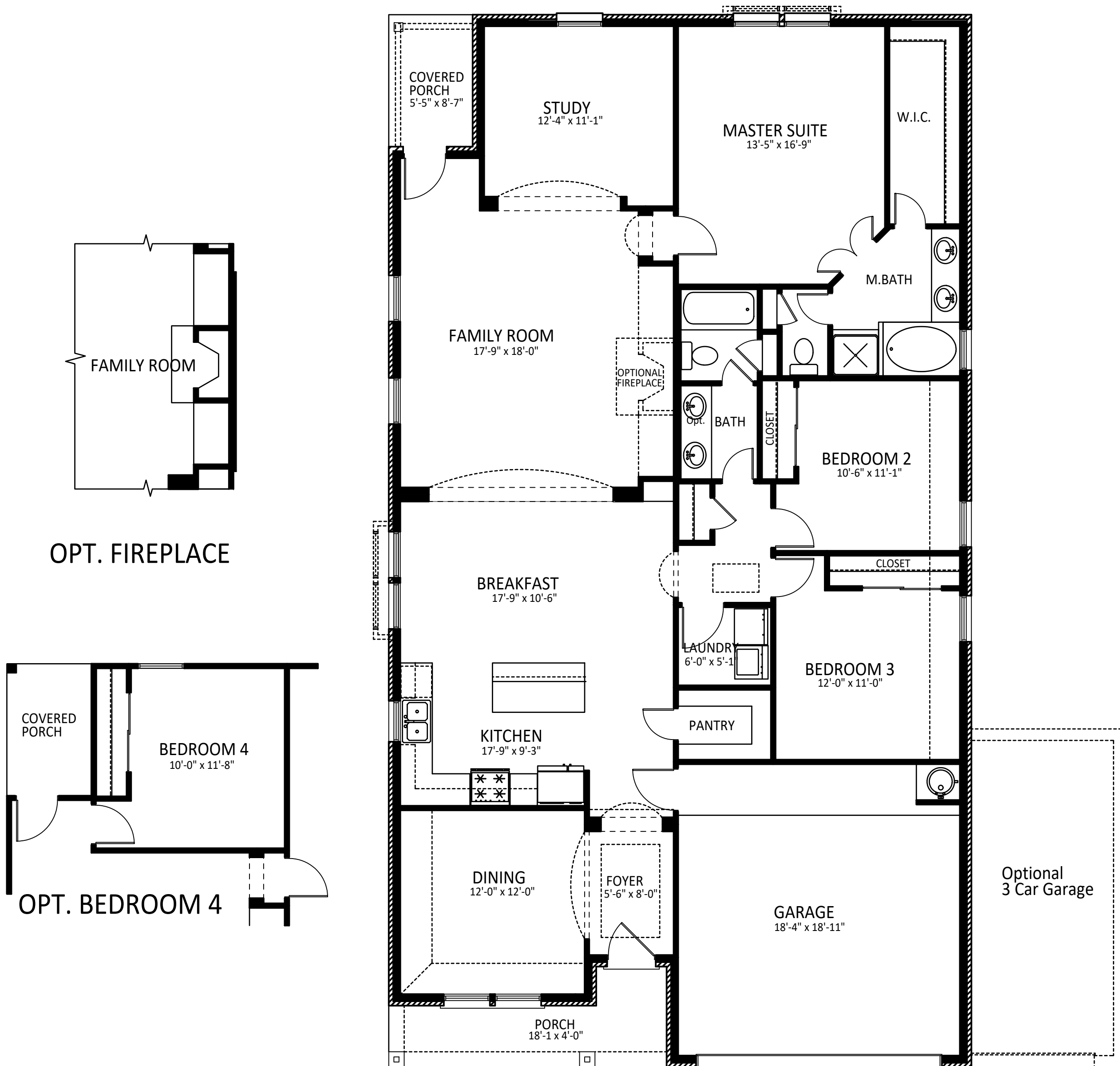
FLOOR PLAN
