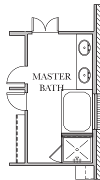
OPT. MASTER BATH TUB / SHOWER
