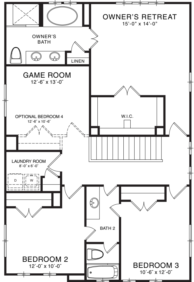
SECOND FLOOR PLAN STYLE A
