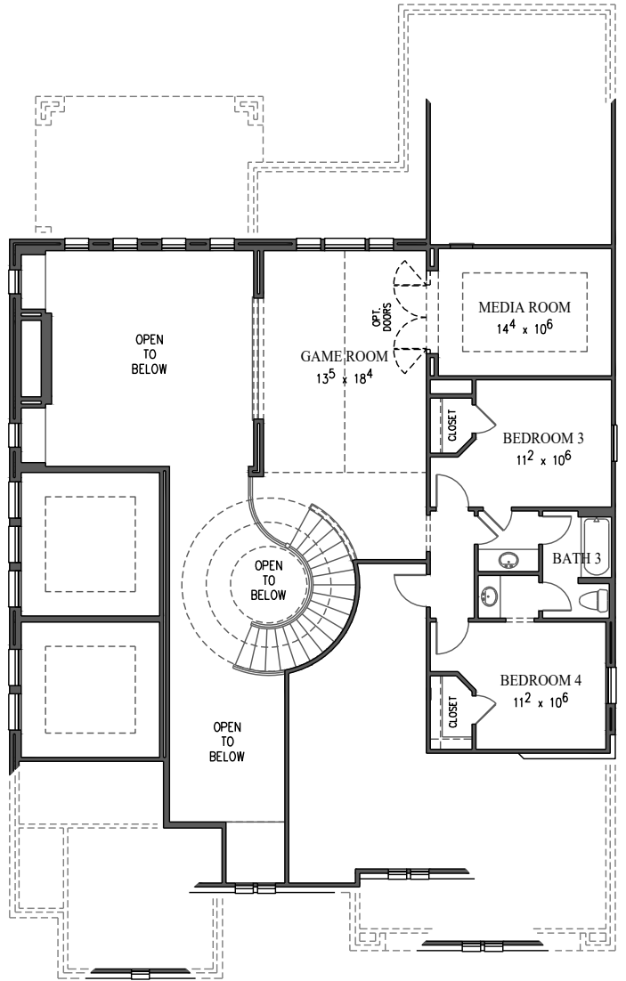
SECOND FLOOR
