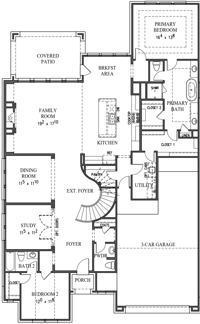
FIRST FLOOR
