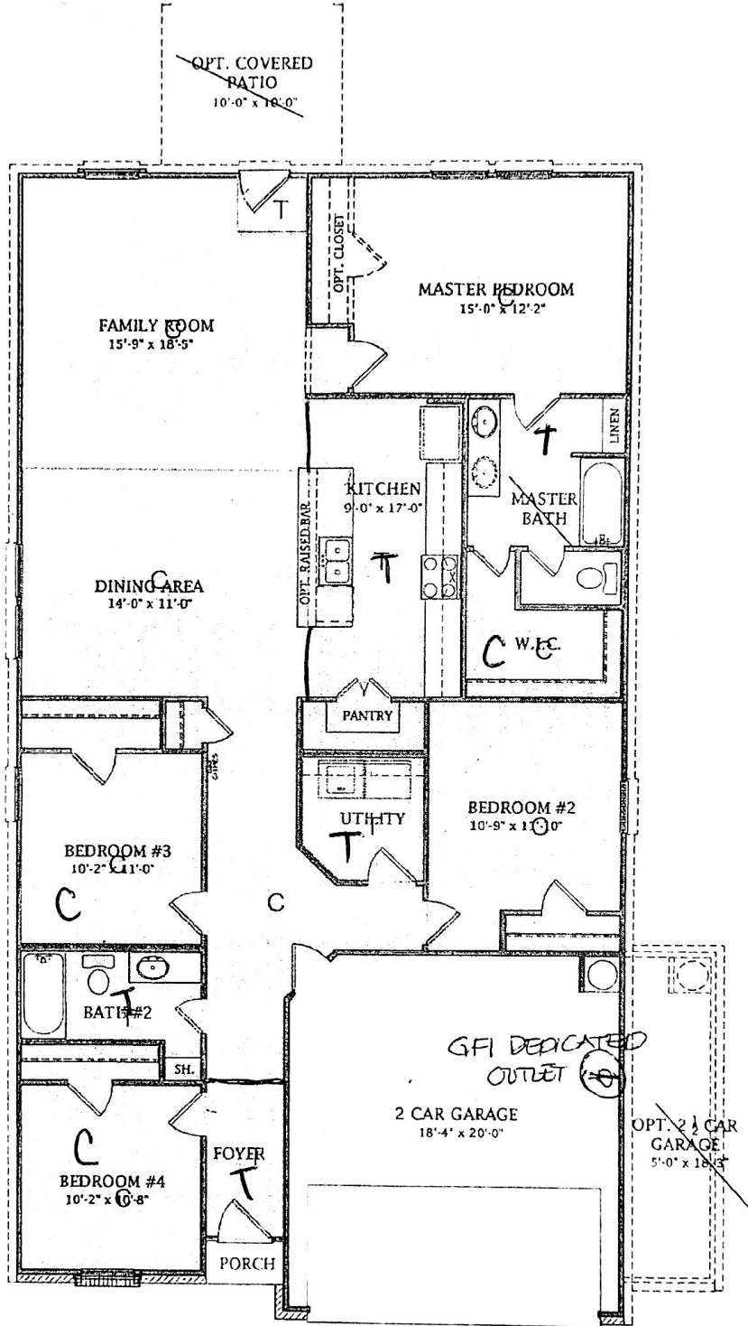
FLOOR PLAN
