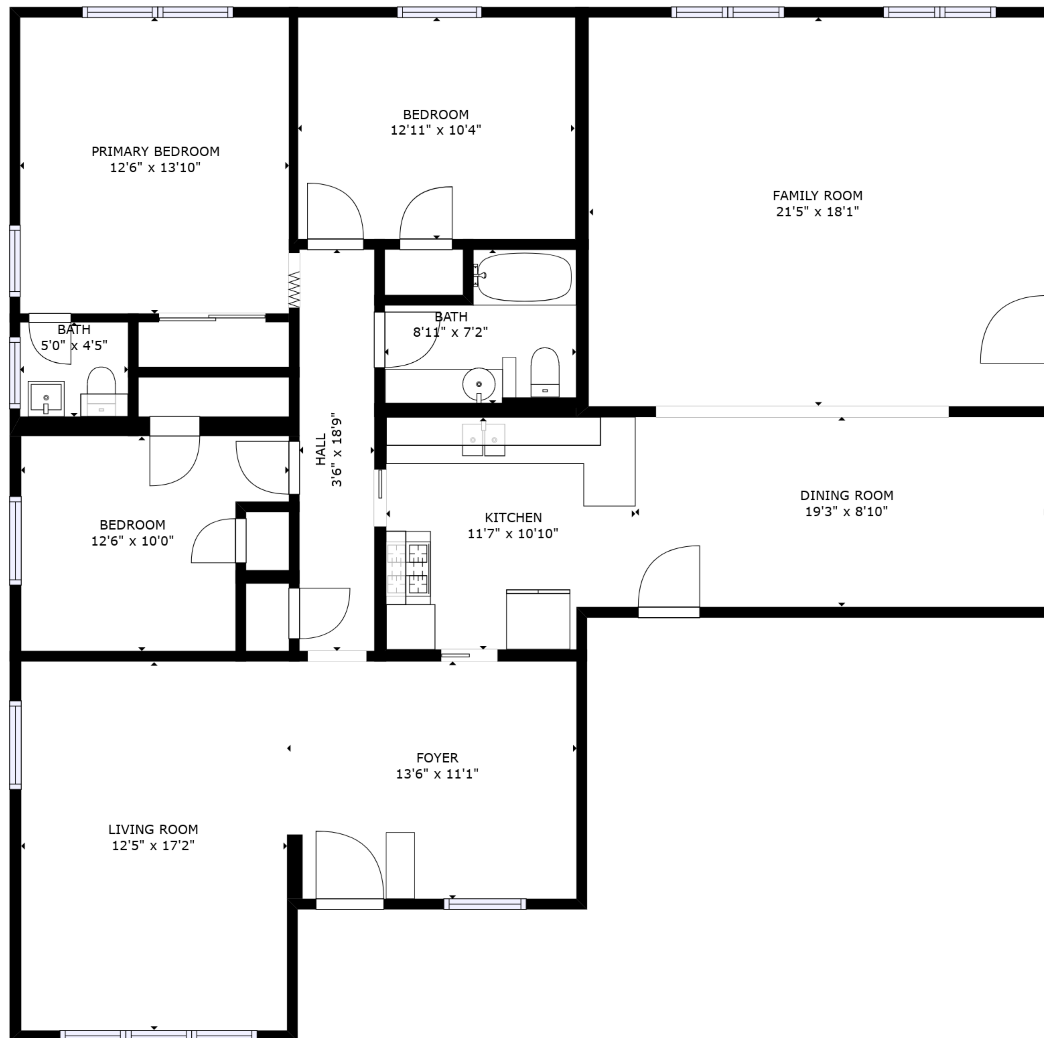
FLOOR 1
