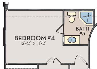
OPT. BATH #3
