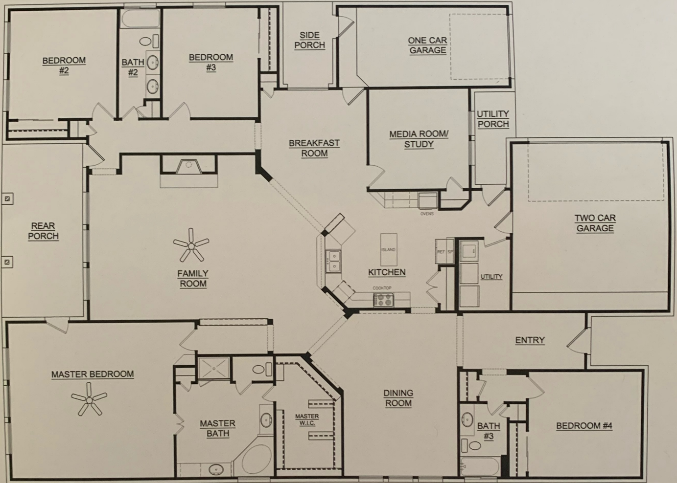
FIRST FLOOR
