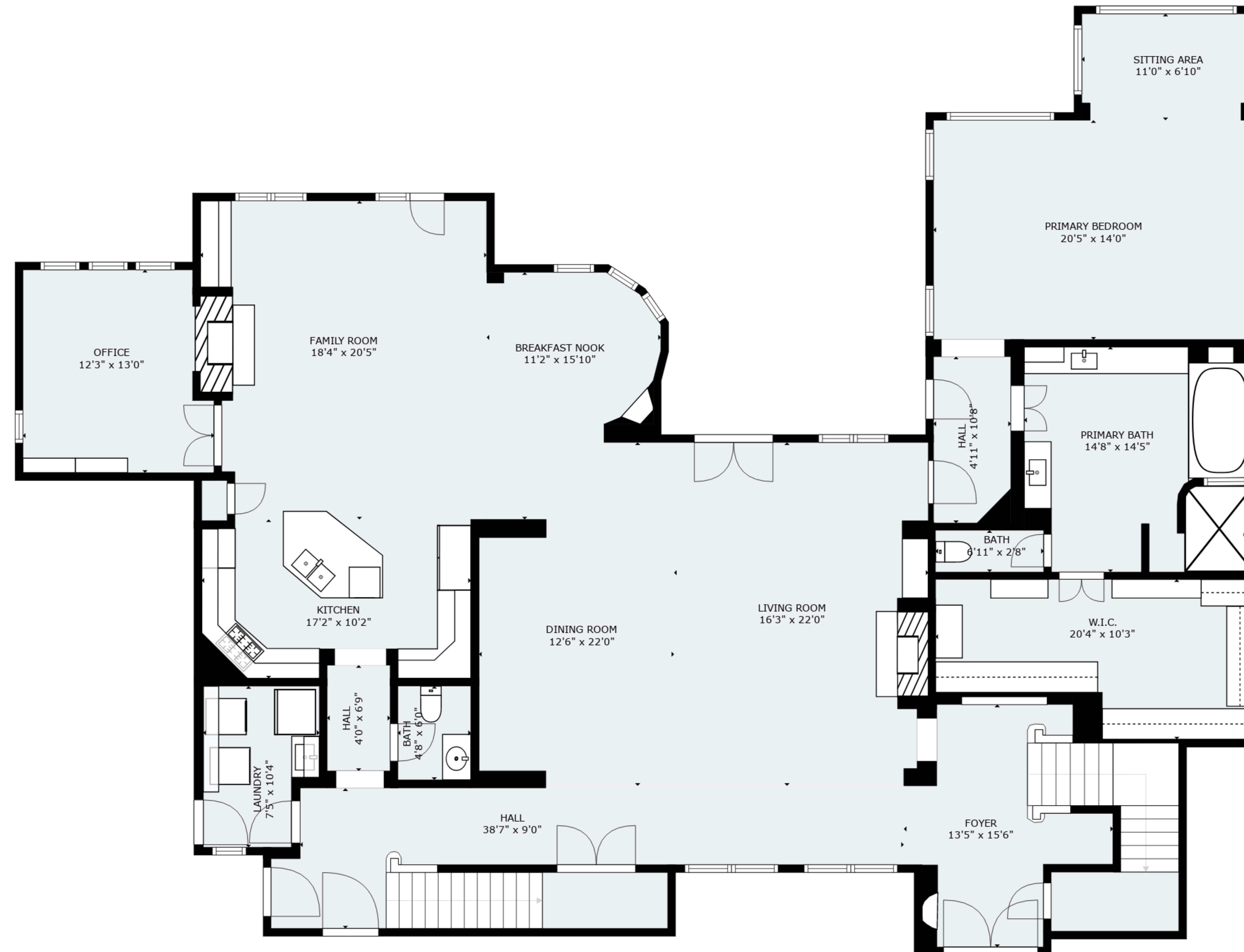
FLOOR 1
