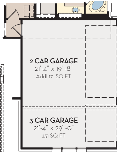
OPT. 2 & 3 CAR SIDE LOAD GARAGE
