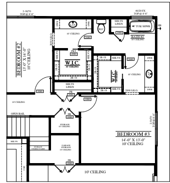
FLOOR PLAN @ OPTIONAL JACK AND JILL BATH
