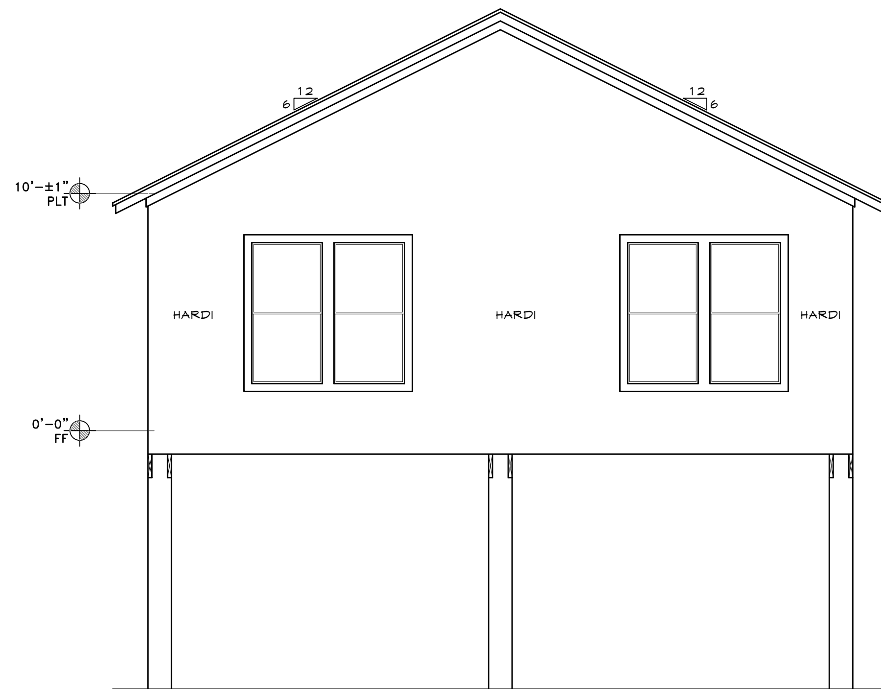
1 REAR VIEW A2 SCALE: 1/4" = 1'
