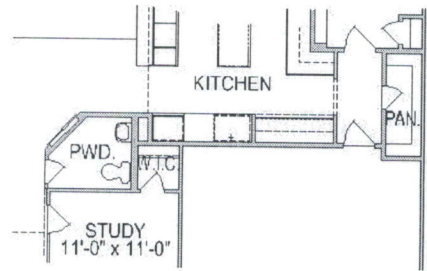
FIRST FLOOR PLAN OPT. #0578 RELOCATE POWDER ROOM
