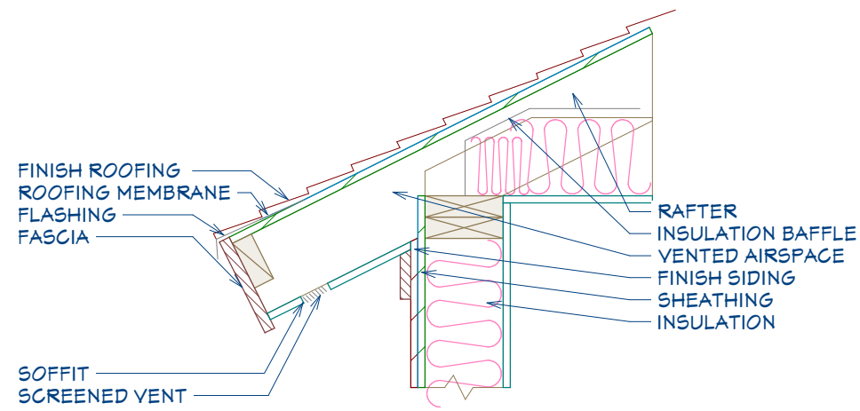
Boxed in Eave SCALE: 1" = 1'
