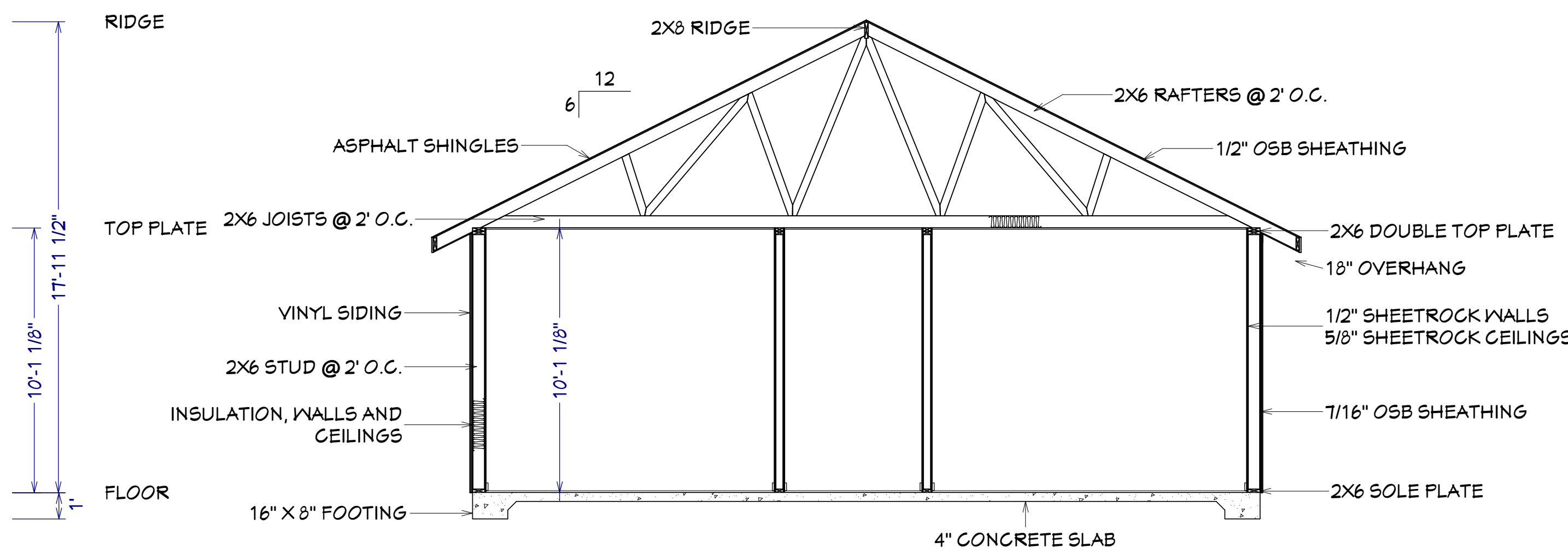
CROSS SECTION SCALE: 1/4" = 1'
