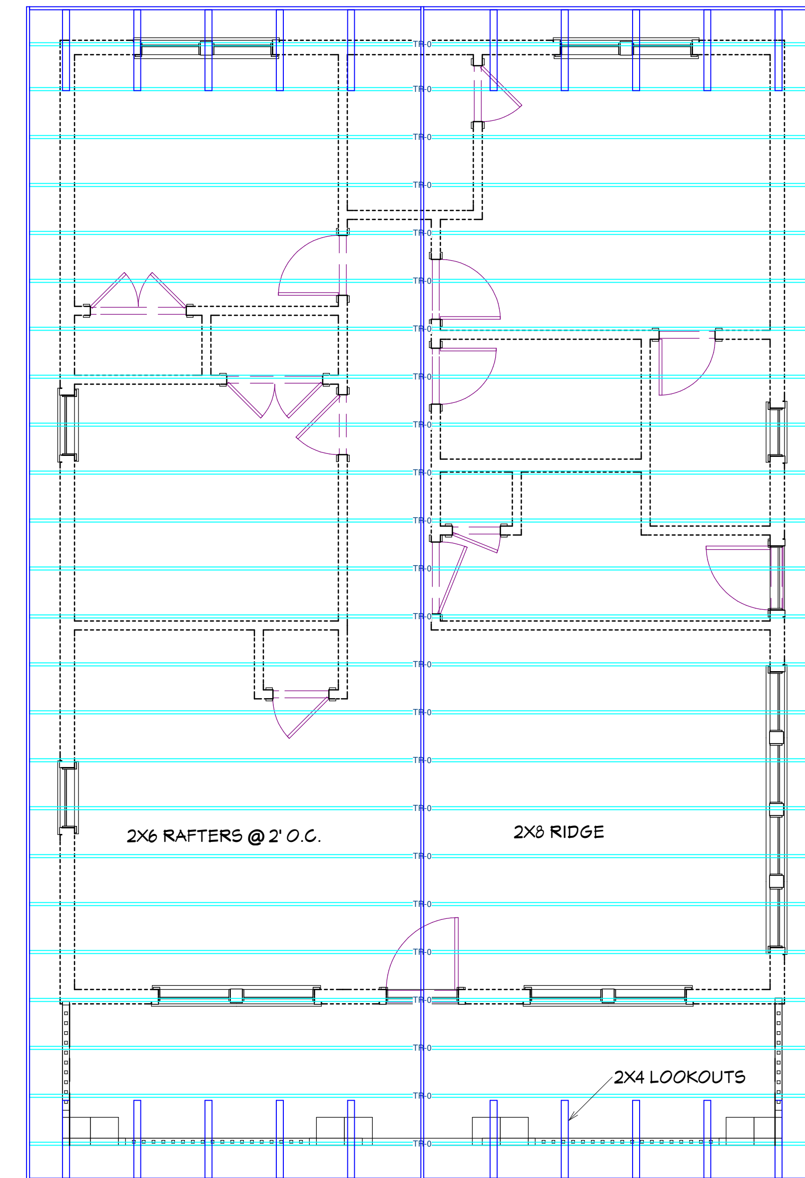
ROOF FRAMING PLAN SCALE: 1/4" = 1'
