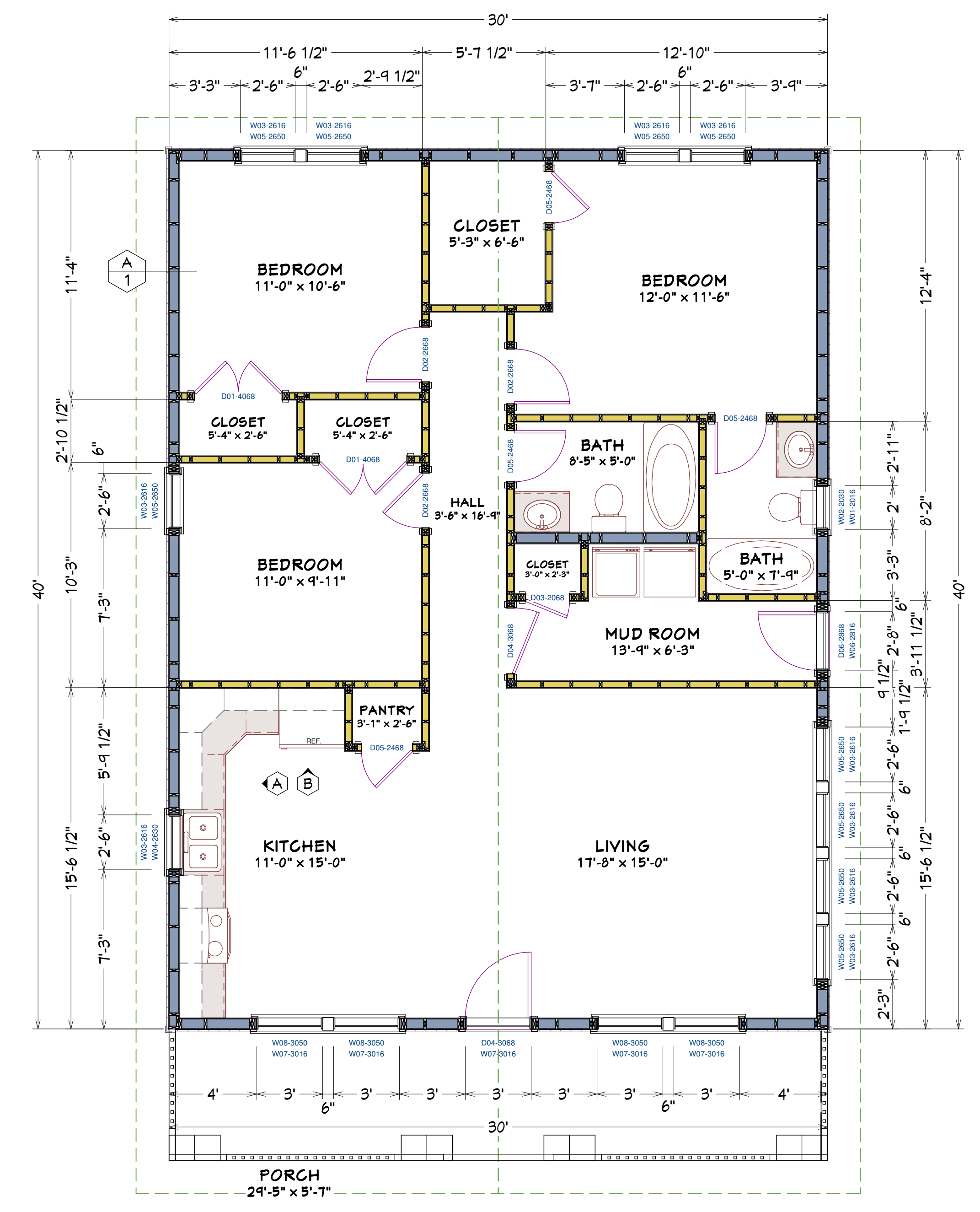
MAIN FLOOR PLAN SCALE: 1/4" = 1'
