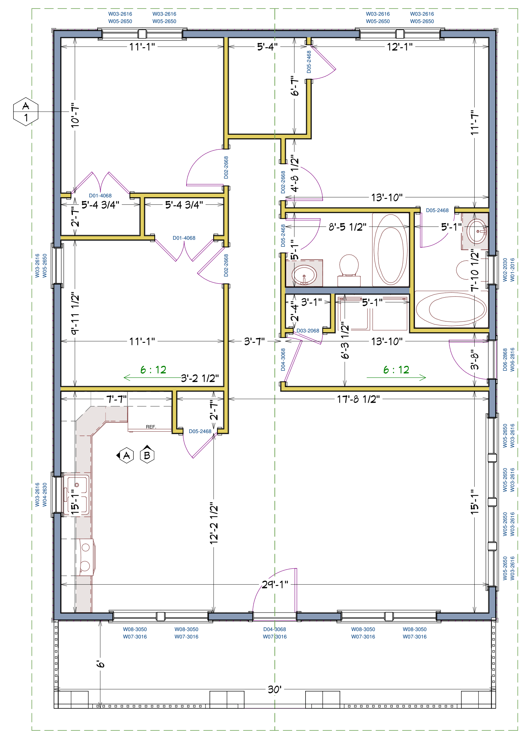
MAIN FLOOR PLAN SCALE: 1/4" = 1'
