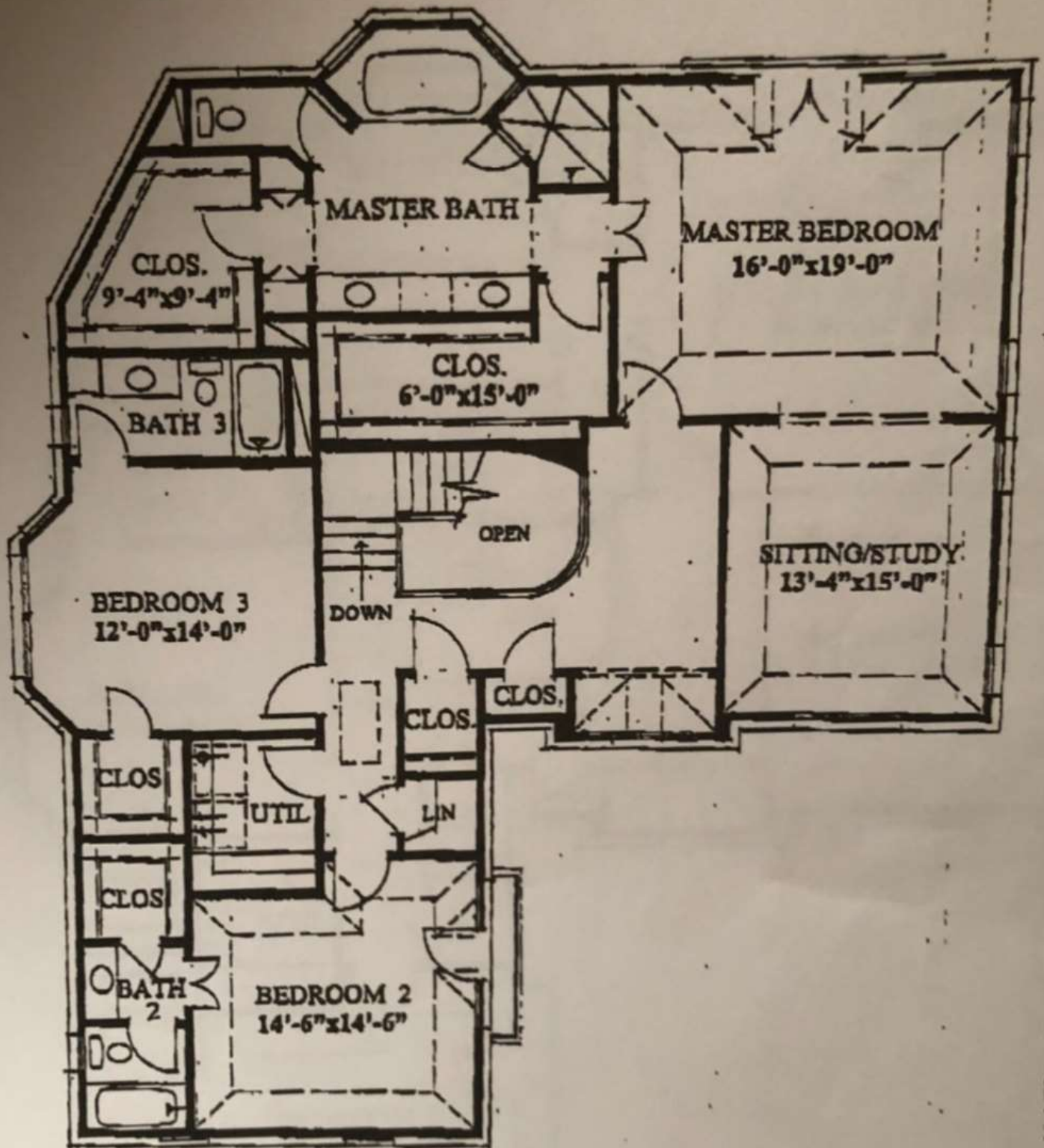
SECOND FLOOR PLAN ALL DIMENSIONS ARE APPROXIMATE
