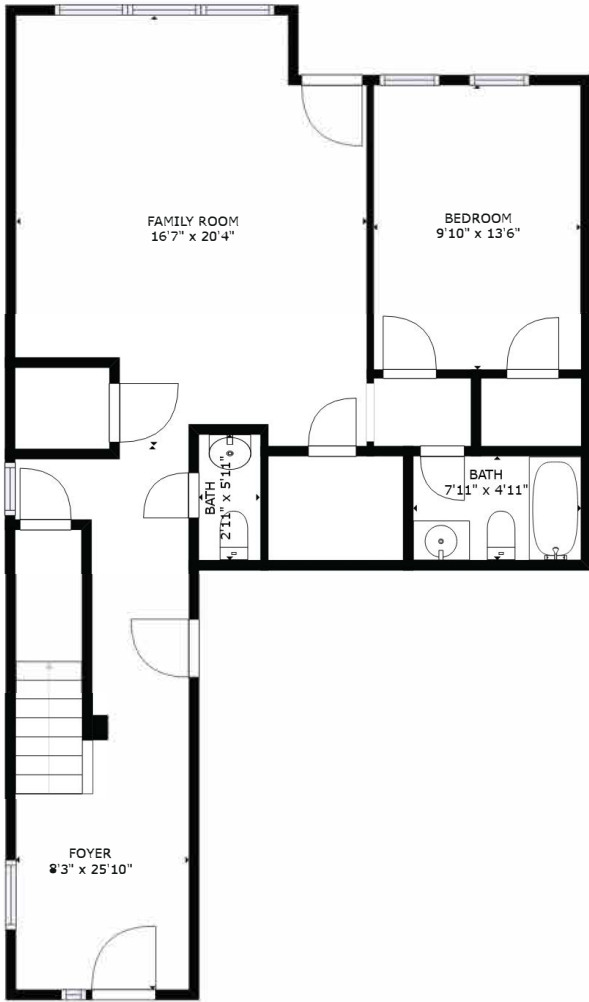
FLOOR 1
