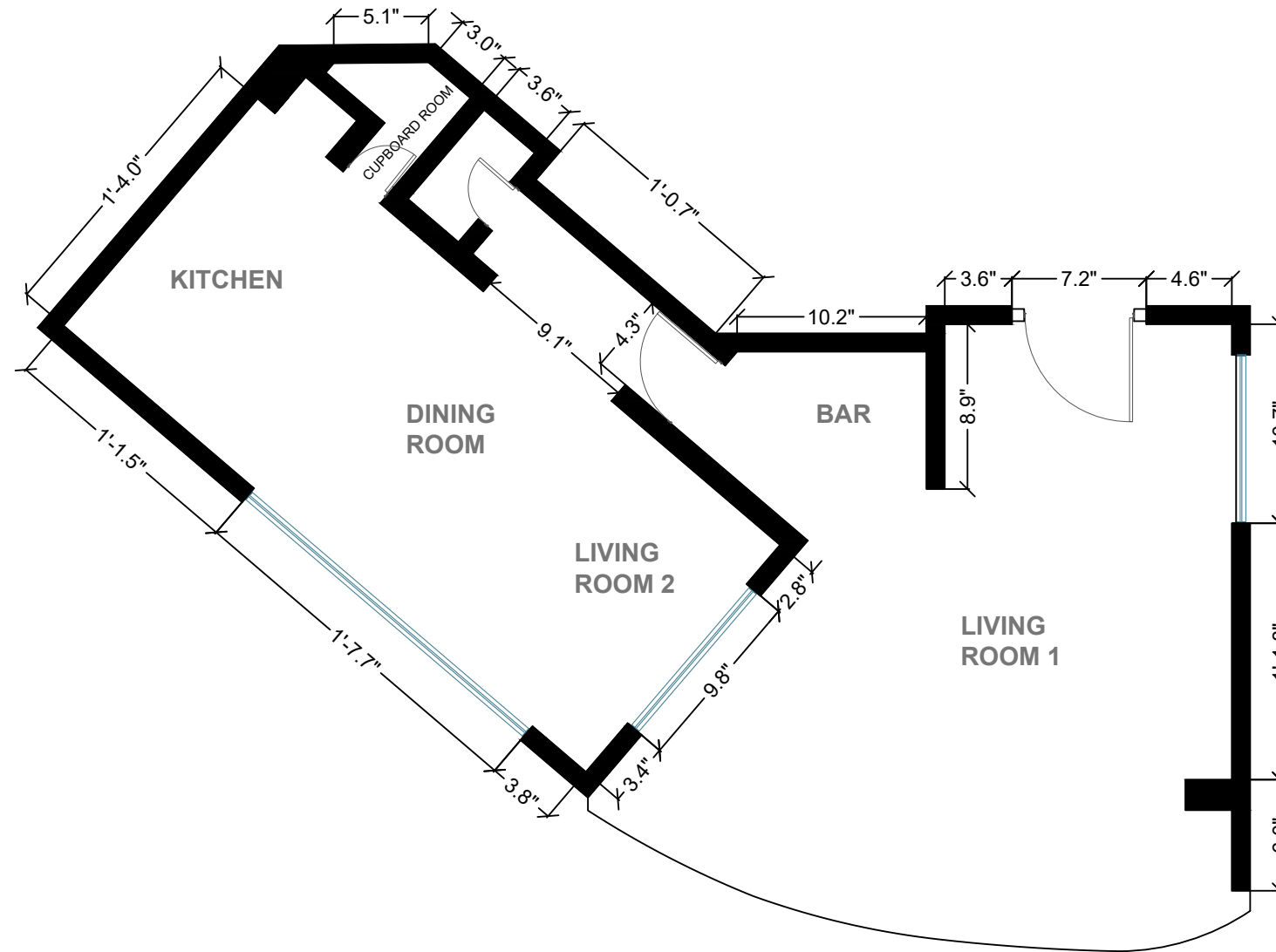
ARCHITECTURAL PLANT - LOW LEVEL SCALE 1:100
