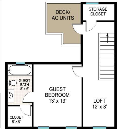
FOURTH FLOOR
