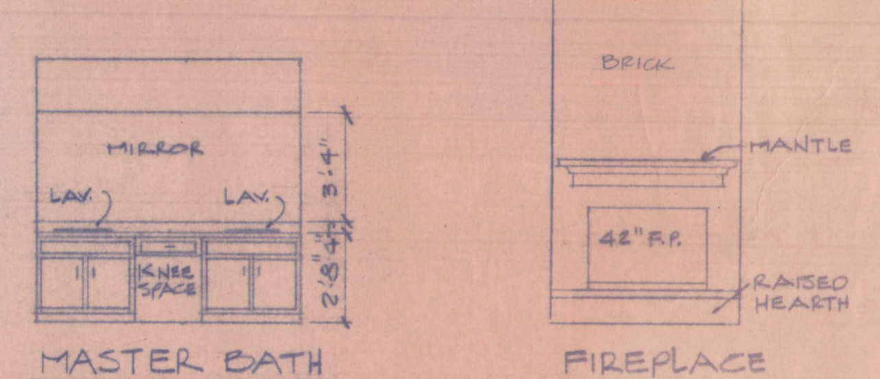
Interior Elevations SCALE 1/4" = 1'-0"
