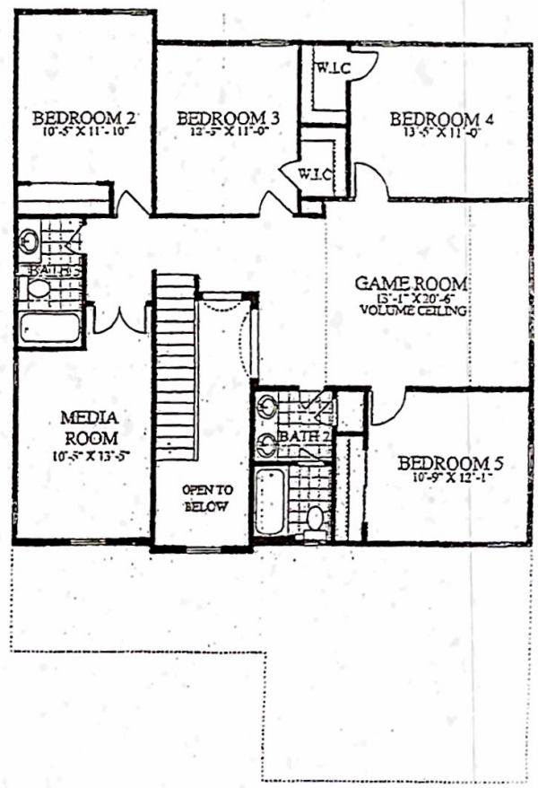
SECOND FLOOR PLAN 1319 S.F.
