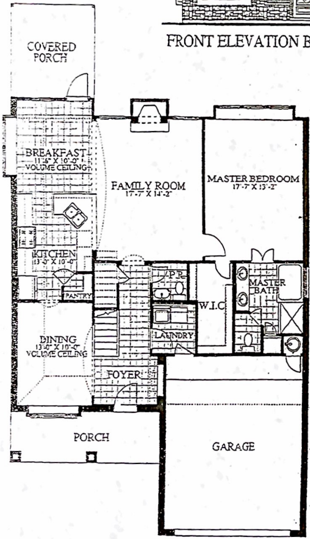
FIRST FLOOR PLAN 1352 S.F.
